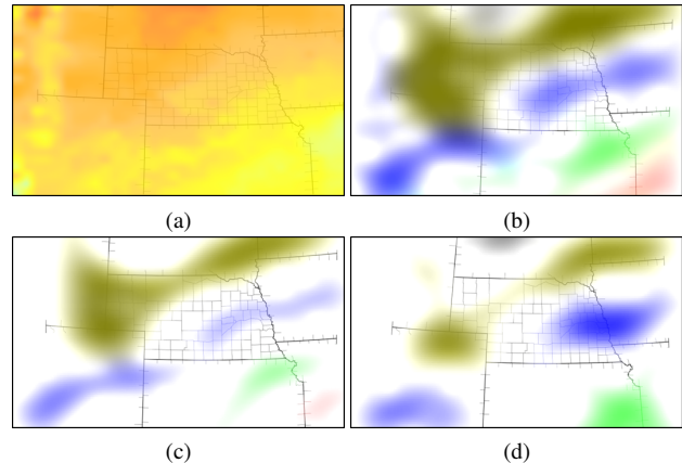
Figure 2. (a) The geographic distribution of TSK variable at a time step. (b) The k-means result with outliers. (c) The comparably dominant weather patterns. (d) The clustering result of the forecasted weather. The color values in (a) are mapped to TSK. The color values in (b)-(d) are used to distinguish different clusters.
