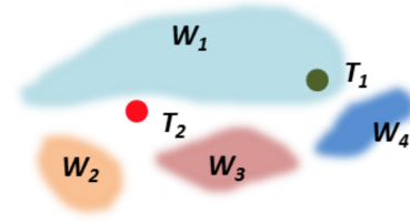
Figure 4. The correlation between the tweets, T_1 and T_2 , and the weather clusters, W_1 , W_2 , W_3 and W_4 . T_1 is highly possible influenced by W_1 whereas T_2 might be related to one of the weathers (i.e. W_1 , W_2 , W_3 ) surrounding it.
