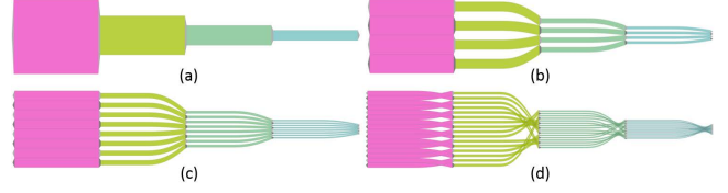
Fig. 5. Processor clustering for binary swap on 16 processors. (a), (b), (c), and (d) show the LOD results with 1, 4, 8, and 16 clusters, respectively, after the bottom-up clustering process. Our method can automatically group the processors into the communication communities, and show the coherent patterns without visual clutter. Our method can achieve the ideal results matching the ground truth of communication pattern without any prior knowledge.
