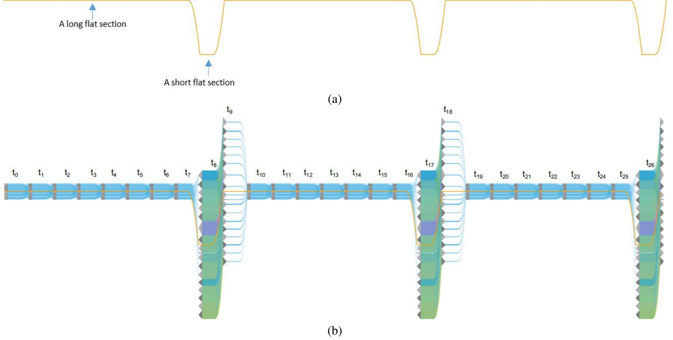
Fig. 7. (a) shows the CommGram curve of the integrated program on 4,320 cores. (b) shows our polygon based visualization.
