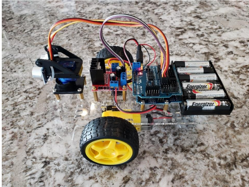
Figure 1: Assembled Robot
