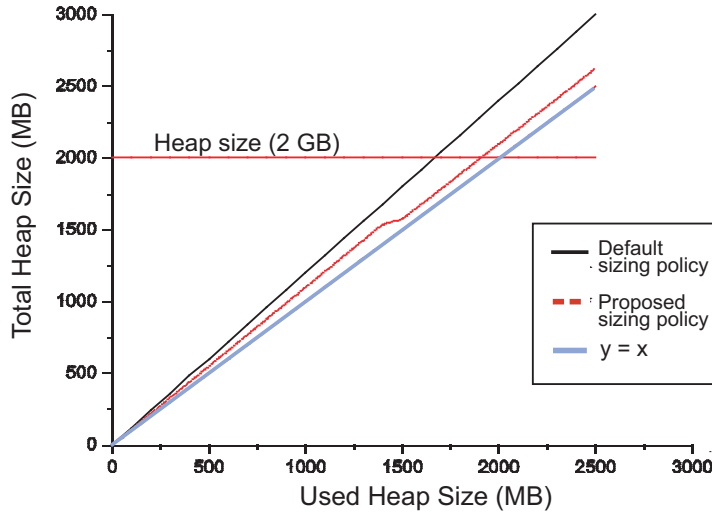
Fig. 12. Heap usage with the adaptive sizing mechanism
