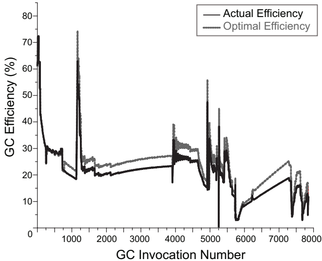
Fig. 17. Identifying efficient garbage collection triggering points
