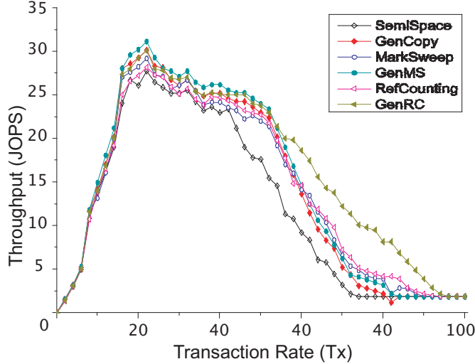
Fig. 15. Comparing the throughputs of different GC techniques
