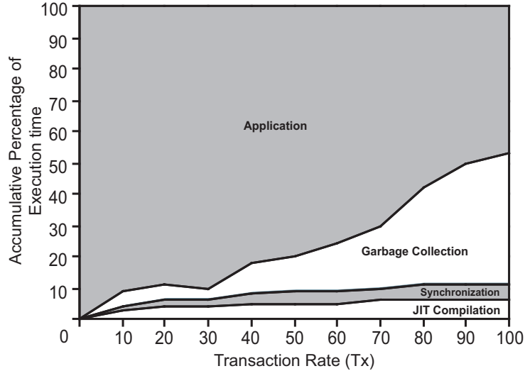
Fig. 4. Accumulative time spent in major runtime functions
