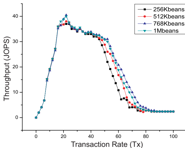
Fig. 16. Effects of varying sizes of object-cache
