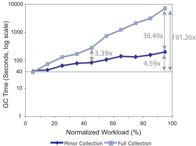
Fig. 6. Time spent in minor GC and full GC
