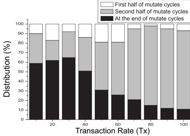
Fig. 10. Execution regions that contain optimal GC invocation points
