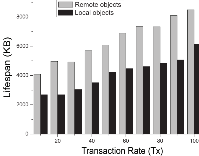
Fig. 8. Comparing life spans of local and remote objects
