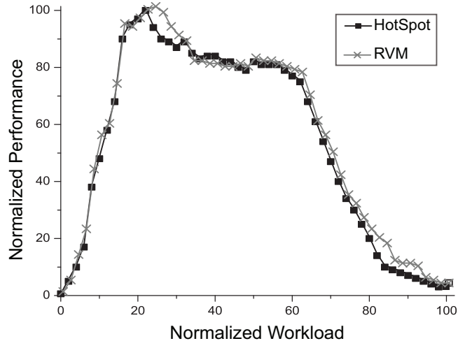
Fig. 14. Comparing throughputs of system_{RVM} to system_{HotSpot}
