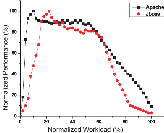
Fig. 2. Throughput degradation behaviors of JBoss and Apache
