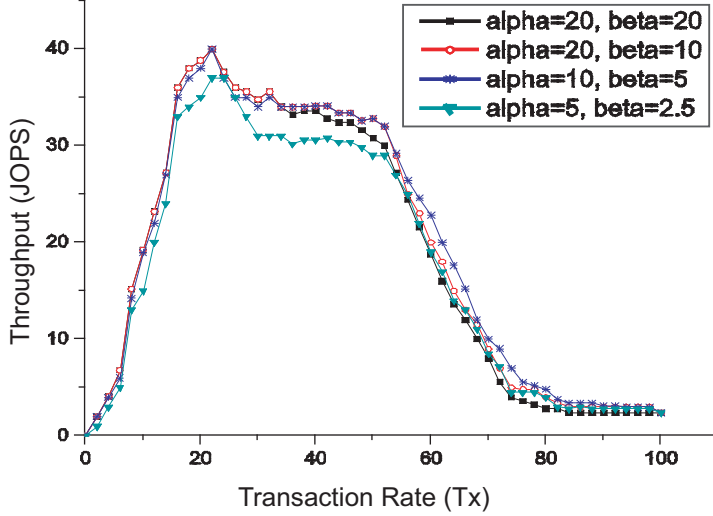
Fig. 11. Throughput performance after applying the adaptive sizing mechanism
