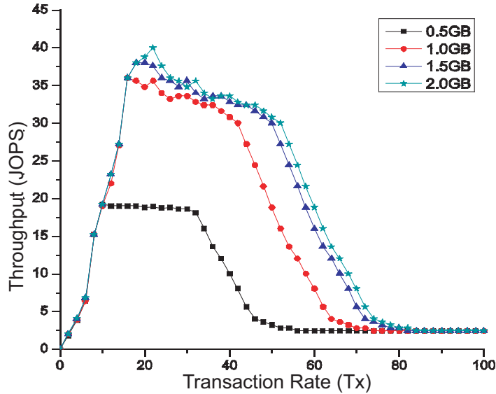
Fig. 3. Throughput comparison with respect to heap sizes
