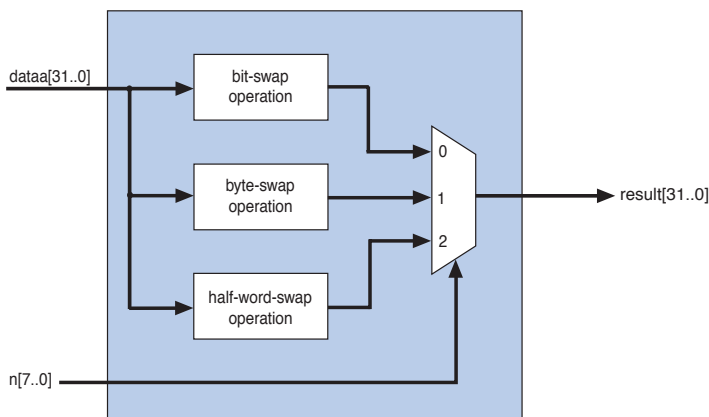
Figure 1–7. Extended Custom Instruction with Swap Operations
