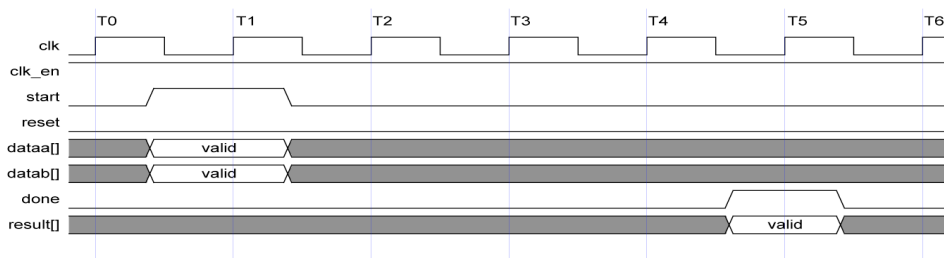
Figure 1–6. Multi-Cycle Custom Instruction Timing Diagram
