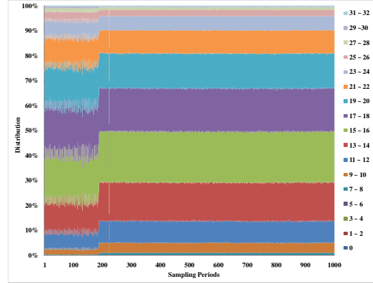
(a) omnetpp
