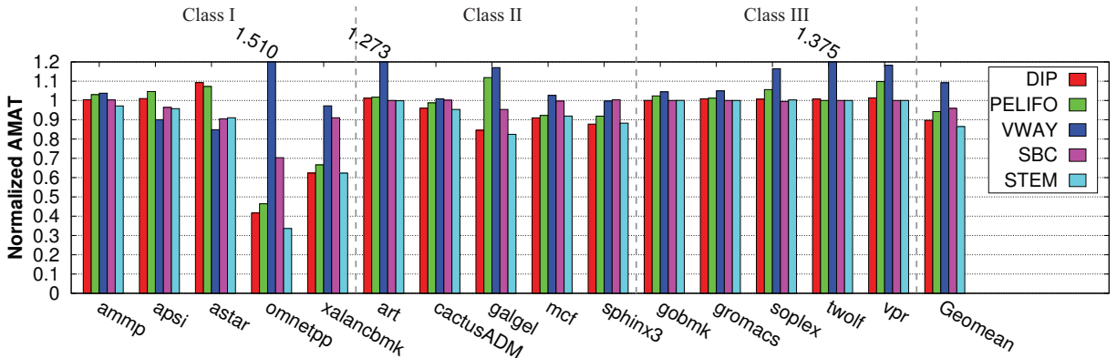
Figure 8. Normalized AMAT
