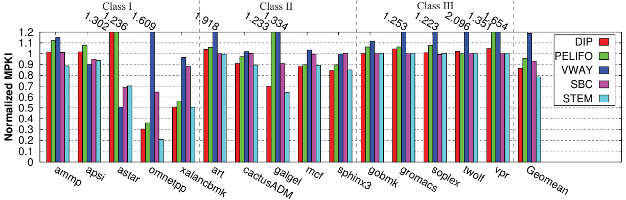
Figure 7. Normalized MPKI
