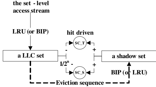
Figure 5. A Set-Level Capacity Demand Monitor (SCDM)
