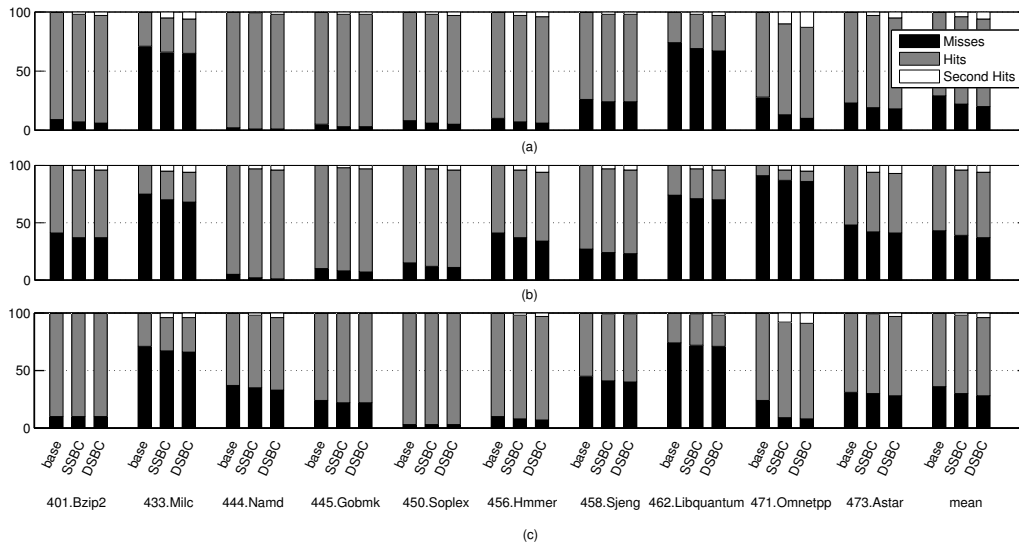
Figure 6: Miss, hit and secondary hit rates for the (a) L2 cache in the two-level configuration, (b) L2 cache in the three-level configuration, and (c) L3 cache in the three-level configuration.
