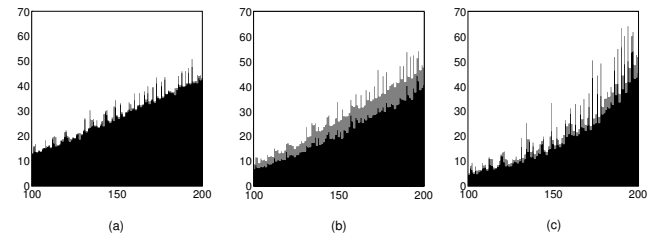
Figure 4: Distribution of the sets with a high saturation level(black), medium saturation level(gray) and low saturation level(white) during a portion of the execution of omnetpp in the L2 cache of the two-level configuration. (a) Baseline (b) Static SBC (c) Dynamic SBC. Samples each 5 * 10^5 K accesses.
