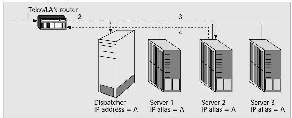
■ Figure 3. Traffic flow in an L4/2 cluster.
