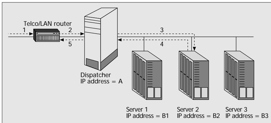
■ Figure 5. Traffic flow in an L4/3 cluster.
