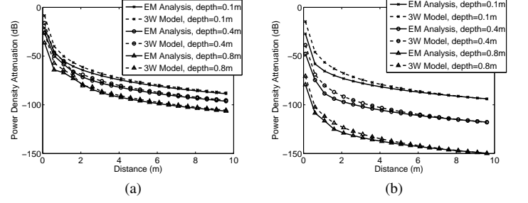
Fig. 2: Comparison of the results of the electromagnetic analysis and the 3W model with different burial depths. (a) VWC=10%; (b) VWC=35%
