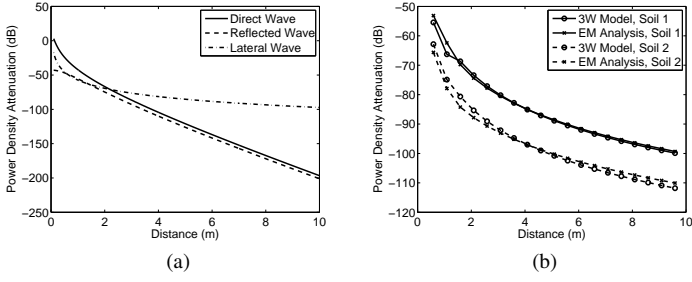
Fig. 3: Analysis of the Model. (a) the comparison of the three components over distance; (b) applying the model to two soil types.
