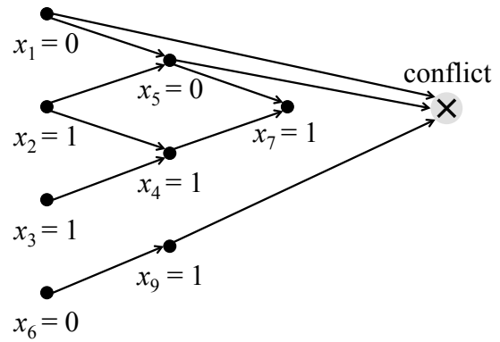
Figure 2: An implication graph that has reached a conflict.
