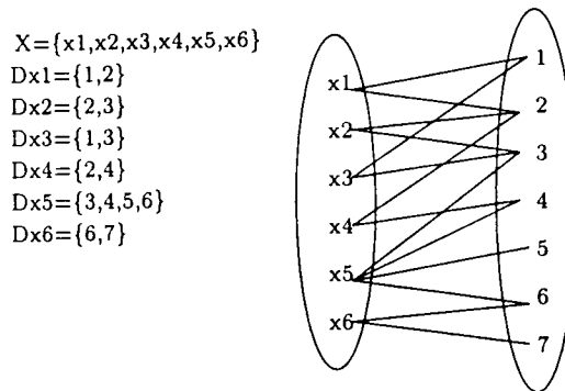
Figure 2: A constraint of difference defined on a set X and its value graph.
