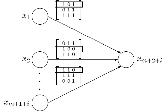
Figure 2: Instantiating x_{m+2+i}
