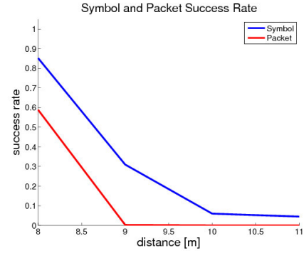
Fig. 8: Singapore Optical Modem Experiment: Long Range symbol and packet success rate using blue light. The x axis corresponds to distance. The y axis shows the percentage of valid pulses received (blue line) and valid packets received (red line).
