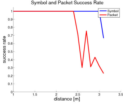
Fig. 6: Singapore Optical Modem Experiment: Short Range symbol and packet success rate using blue light. The x axis corresponds to distance. The y axis shows the percentage of valid pulses received (blue line) and valid packets received (red line).
