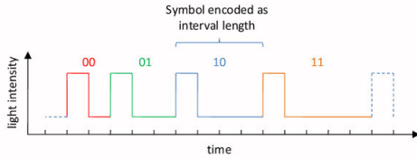
Fig. 2: DPIM (discrete pulse interval modulation): Each bit-pair is represented by a different distance between two successive light pulses.
