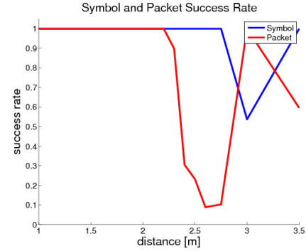
Fig. 5: Singapore Optical Modem Experiment: Short Range symbol and packet success rate using green light. The x axis corresponds to distance. The y axis shows the percentage of valid pulses received (blue line) and valid packets received (red line).
