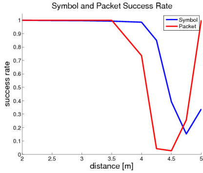
Fig. 9: Singapore Optical Modem Experiment: Hybrid Modem success rates using the long range optical modem sender and the sort range optical modem receiver using blue light. The x axis corresponds to distance. The y axis shows the percentage of valid pulses received (blue line) and valid packets received (red line).
