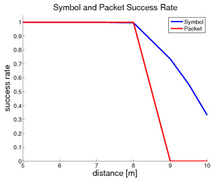
Fig. 7: Singapore Optical Modem Experiment: Long Range symbol and packet success rate using blue light. The x axis corresponds to distance. The y axis shows the percentage of valid pulses received (blue line) and valid packets received (red line).
