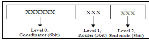
Figure 2. Addressing buffer
