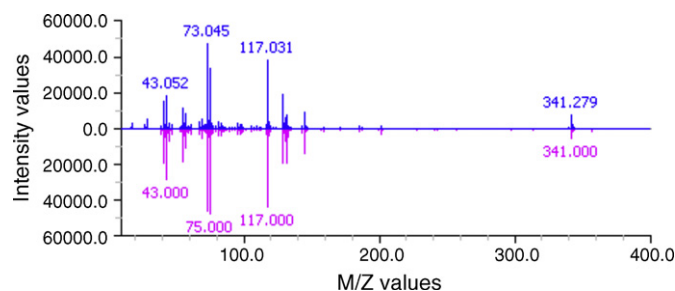
Fig. 7. Mass spectrum for a detected blob (top, in blue) head-to-tail with the Manchester Metabolomics Database mass spectrum for stearic acid TMS [22] (bottom, in magenta). (For interpretation of the references to color in this figure legend, the reader is referred to the web version of the article.)
