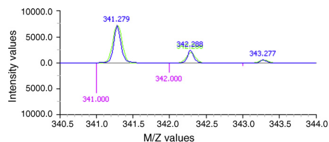
Fig. 8. Selected ion peaks from the blob mass spectrum shown in Fig. 7 (top, in blue) head-to-tail with the Manchester Metabolomics Database mass spectrum for stearic acid TMS [22] (bottom, in magenta) and the expected isotopic peaks for C_{20}H_{42}O_2Si^+ (top, overlaid, in green).
