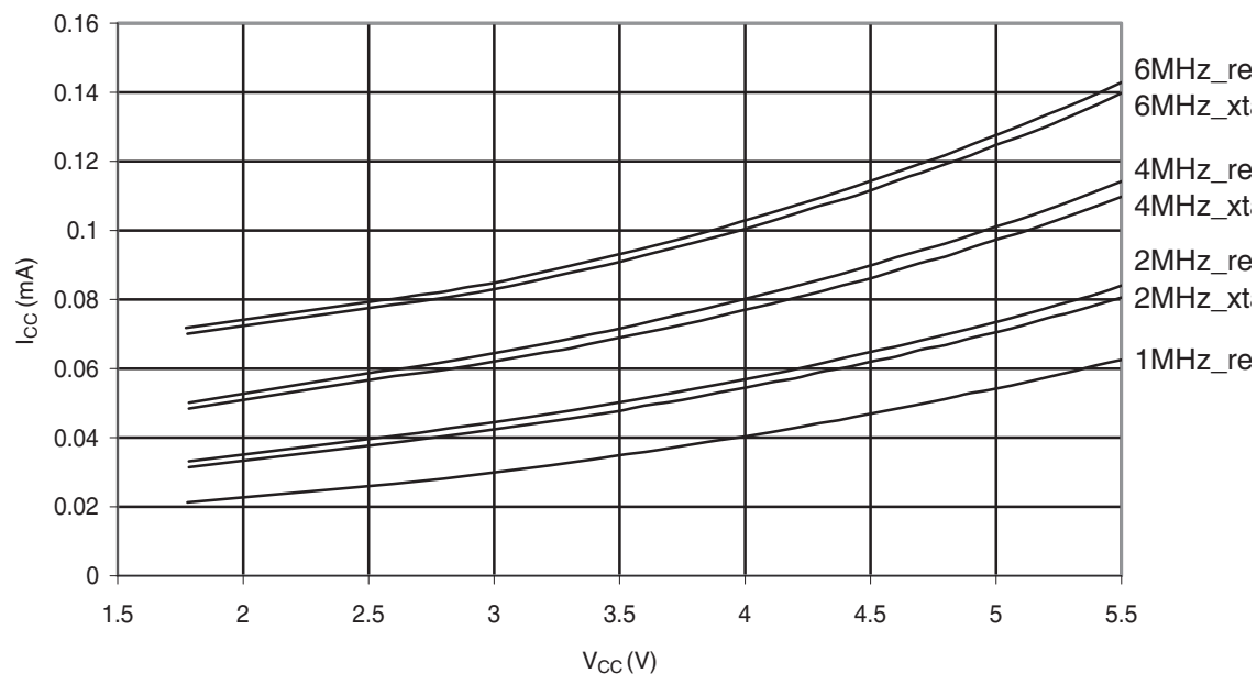
Figure 30-296. ATmega328: Standby Supply Current vs. V_{CC} (Watchdog Timer Disabled)
