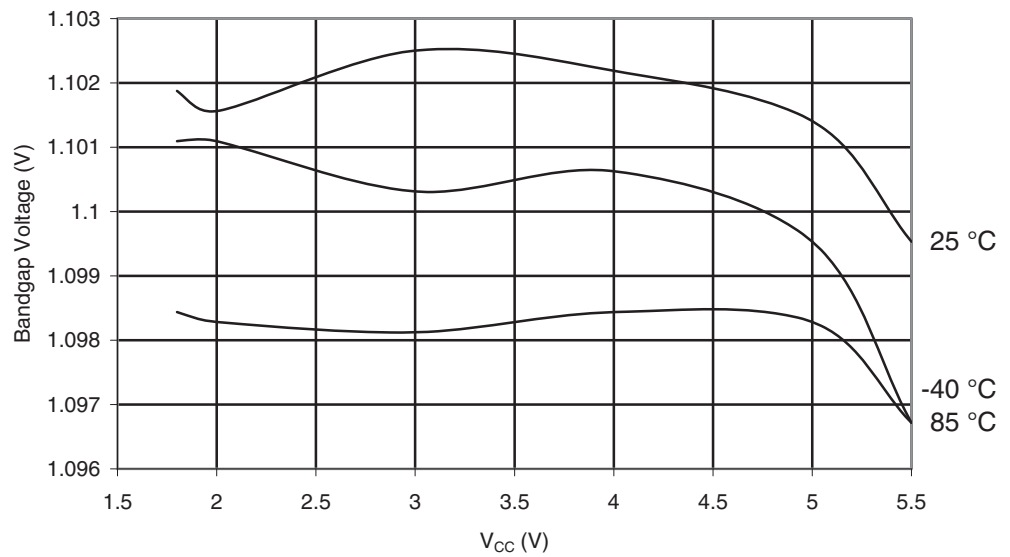
Figure 30-128. ATmega88A: Bandgap Voltage vs. V CC
