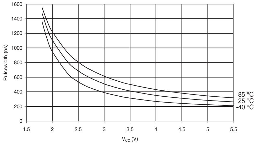
Figure 30-94. ATmega48PA: Minimum Reset Pulse width vs. V_{CC}
