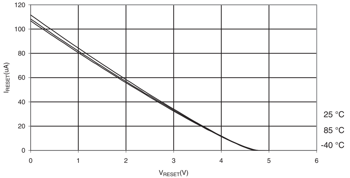
Figure 30-349. ATmega328P: Reset Pull-up Resistor Current vs. Reset Pin Voltage ( V_{CC} = 5\text{ V} )
