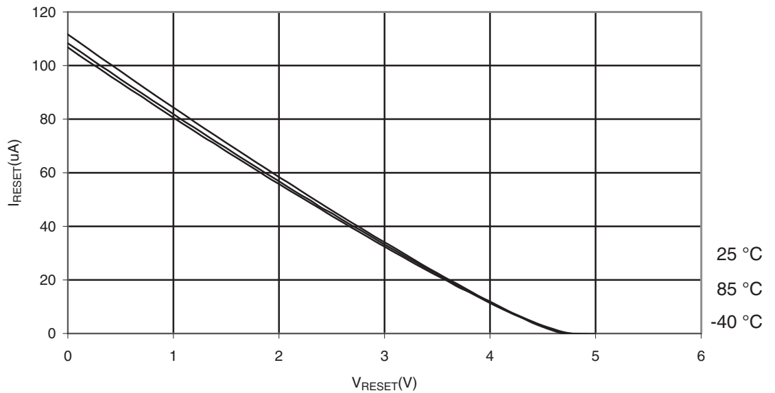
Figure 30-302. ATmega328: Reset Pull-up Resistor Current vs. Reset Pin Voltage ( V_{CC} = 5\text{ V} )
