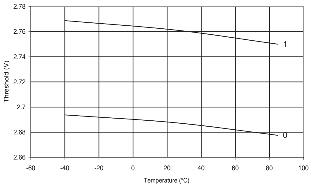
Figure 30-361. ATmega328P: BOD Thresholds vs. Temperature (BODLEVEL is 2.7 V)
