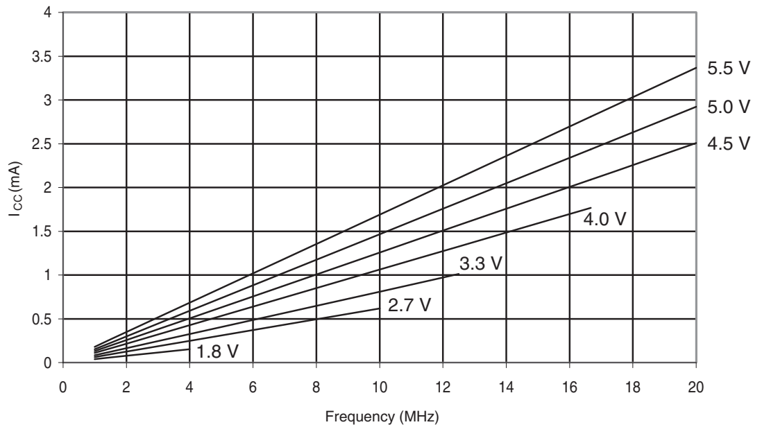
Figure 30-336. ATmega328P: Idle Supply Current vs. Frequency (1-20MHz)
