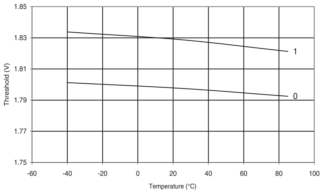
Figure 30-360. ATmega328P: BOD Thresholds vs. Temperature (BODLEVEL is 1.8 V)
