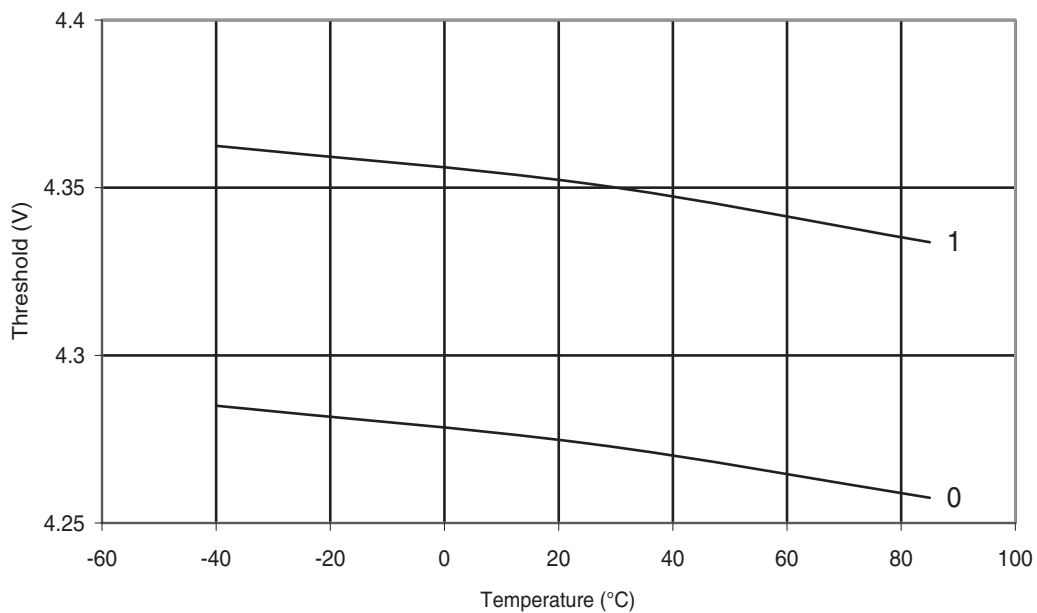
Figure 30-315. ATmega328: BOD Thresholds vs. Temperature (BODLEVEL is 4.3 V)
