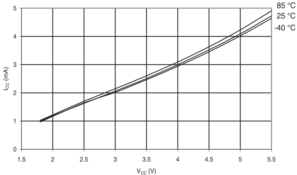
Figure 30-146. ATmega88PA: Active Supply Current vs. V_{CC} (Internal RC Oscillator, 8MHz)
