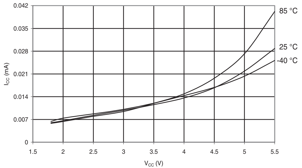
Figure 30-8. ATmega48A: Idle Supply Current vs. V_{CC} (Internal RC Oscillator, 128kHz)
