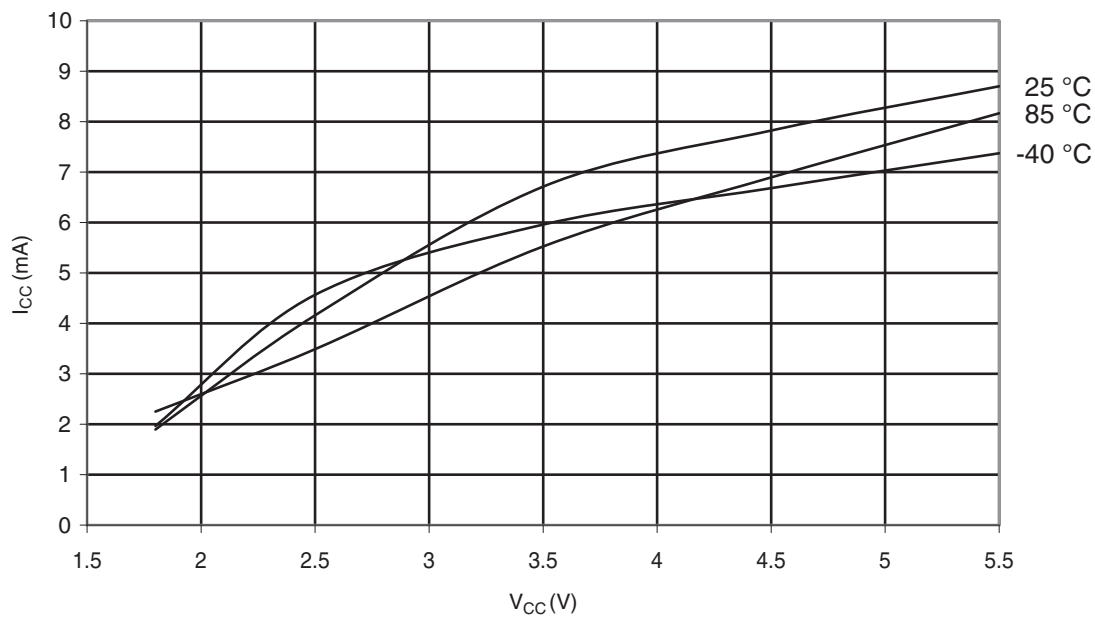
Figure 30-373. ATmega328P: Programming Current vs. V_{CC}
