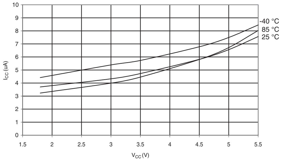
Figure 30-341. ATmega328P: Power-Down Supply Current vs. V_{CC} (Watchdog Timer Enabled)
