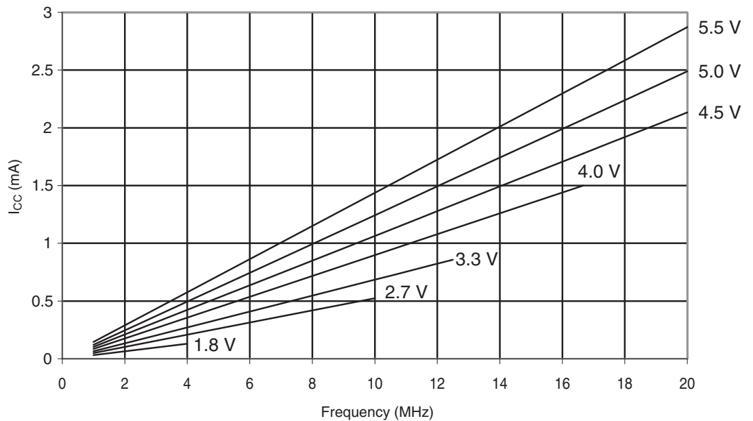
Figure 30-375. ATmega328P: Reset Supply Current vs. Frequency (1 - 20MHz)
