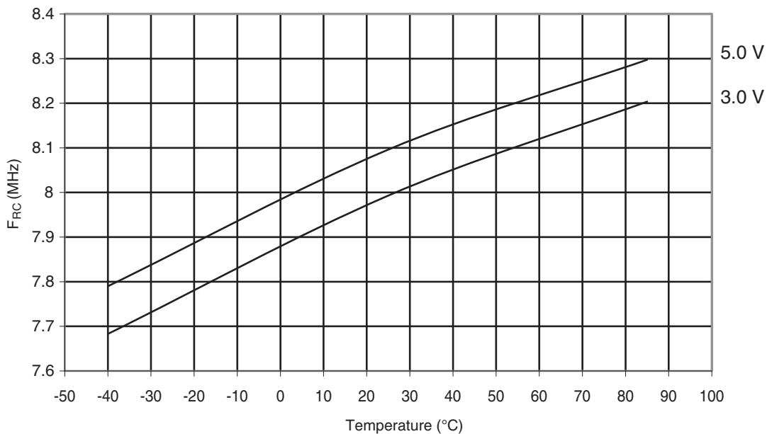
Figure 30-367. ATmega328P: Calibrated 8MHz RC Oscillator Frequency vs. Temperature
