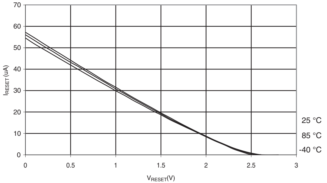
Figure 30-301. ATmega328: Reset Pull-up Resistor Current vs. Reset Pin Voltage ( V_{CC} = 2.7\text{ V} )
