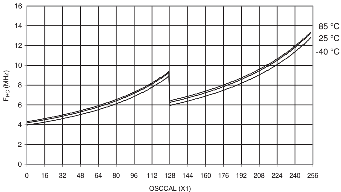
Figure 30-368. ATmega328P: Calibrated 8MHz RC Oscillator Frequency vs. OSCCAL Value
