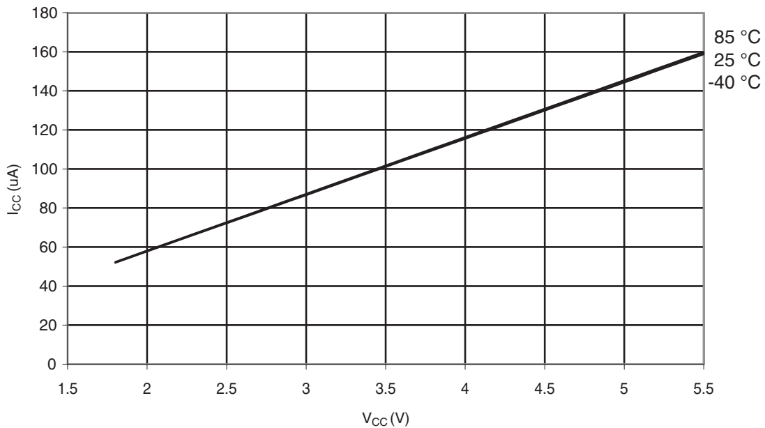
Figure 30-371. ATmega328P: AREF External Reference Current vs. V_{CC}
